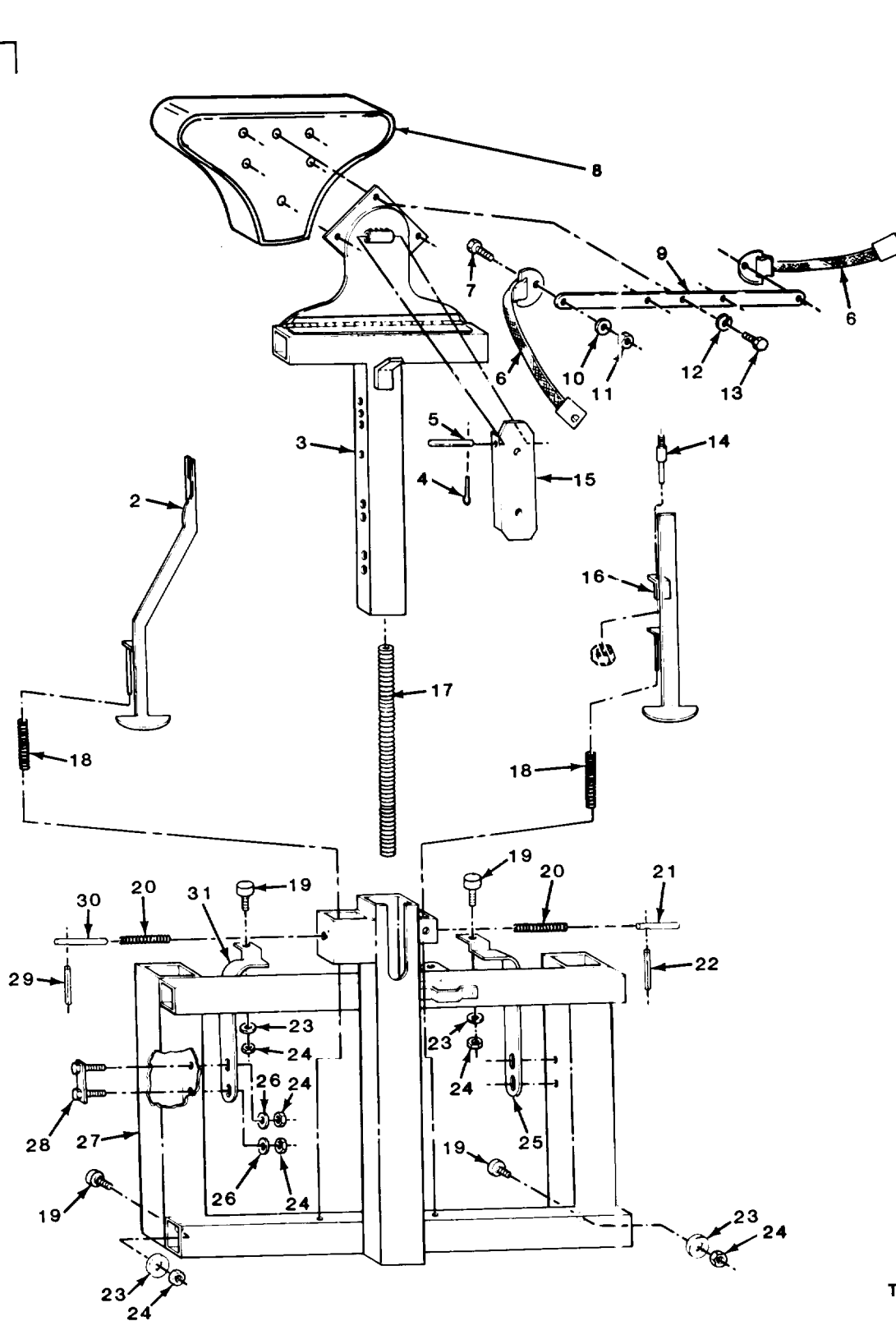
FIGURE 188. ATTENDANT'S SEAT ASSEMBLY AND COMPONENT PARTS (M1010).
