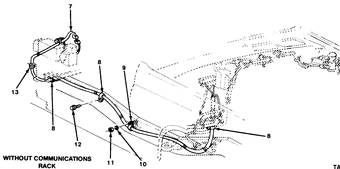
FIGURE 226. PERSONNEL HEATER WIRING HARNESS.
