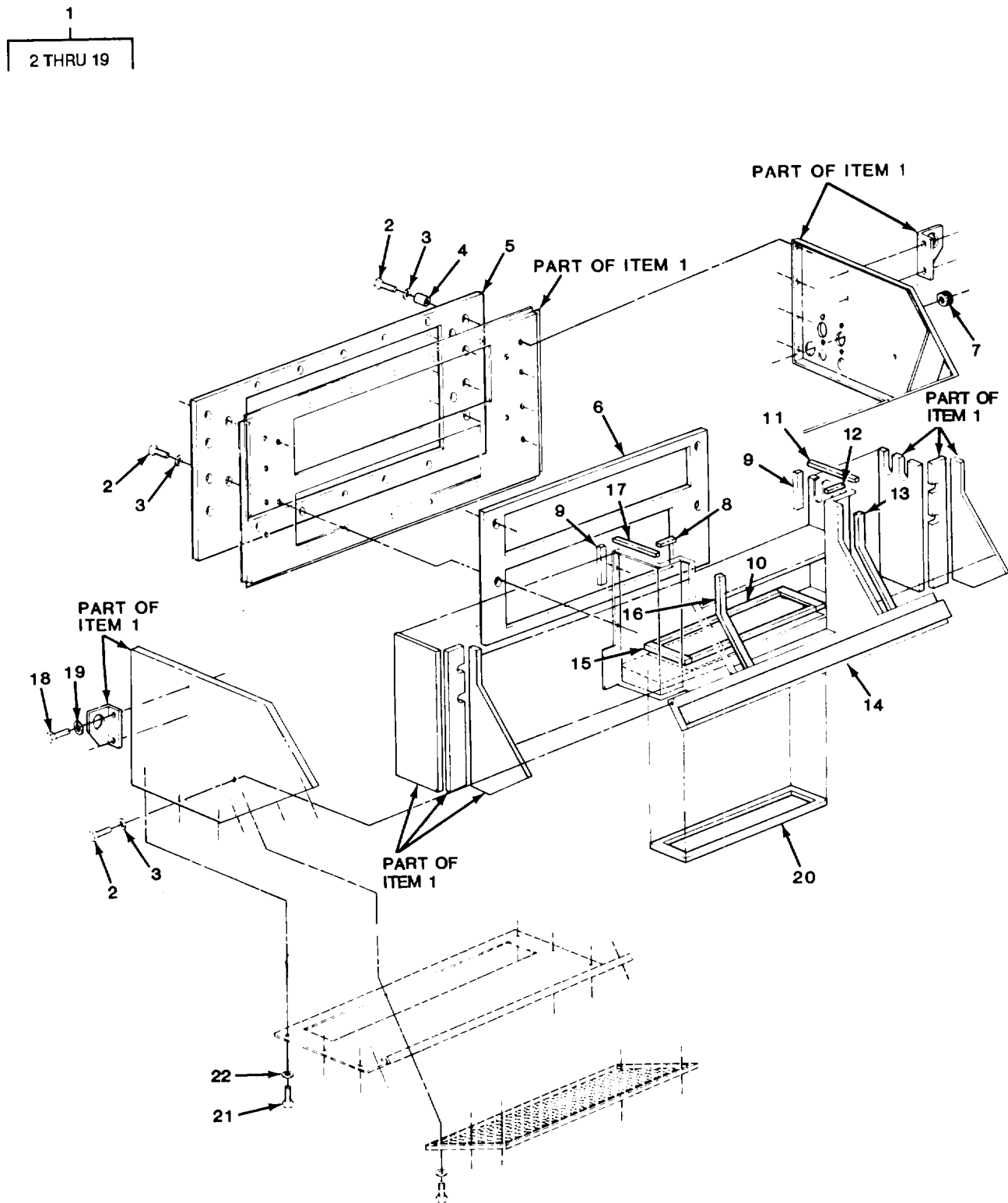
FIGURE 250. MAIN CASE ASSEMBLY AND COMPONENT PARTS (M1010).
