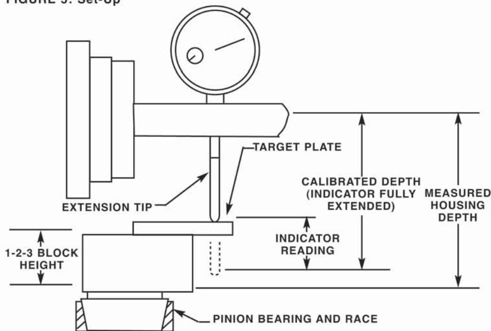
FIGURE 5: Set-Up
